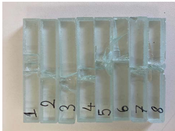
Fig. 3. Laminated glass specimens after impact
