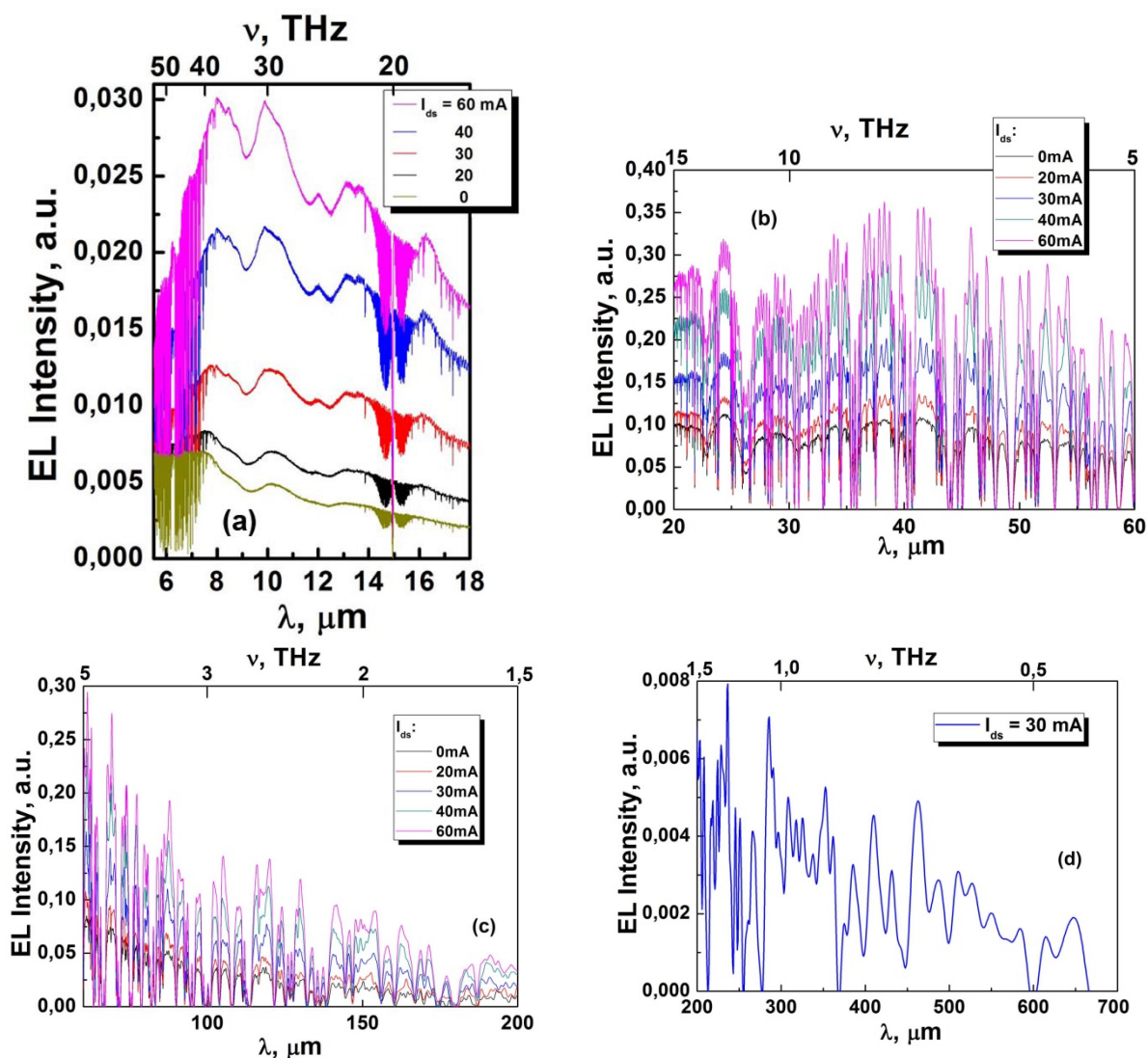
Fig. 3. The full spectra of THz irradiation generated by the therapeutic equipment "IR-Dipole" and "Infrateratron" at various operating currents. Spectra obtained using IR-Fourier spectrometer Bruker-Physik VERTEX 70
