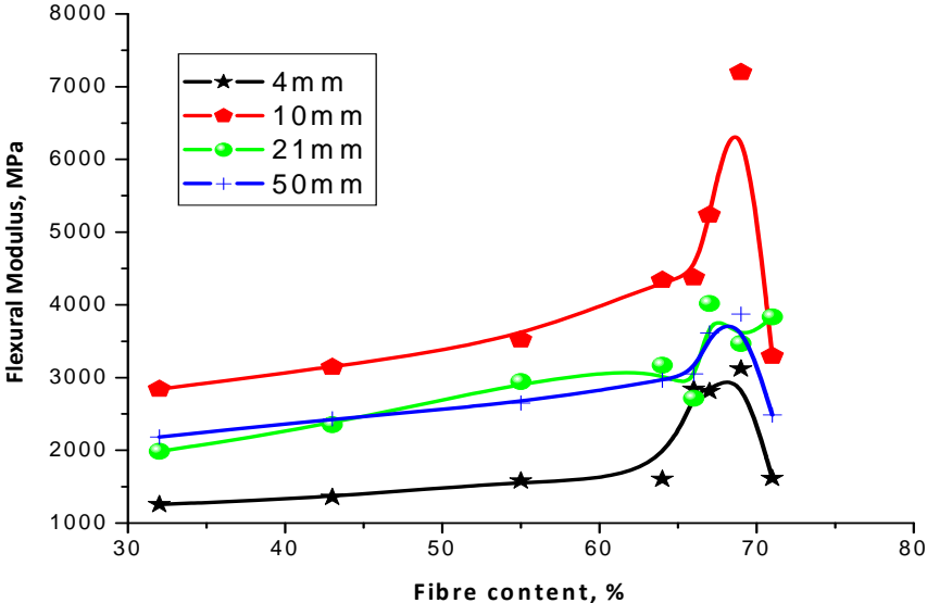
Fig. 7. Flexural modulus of basalt short fibre composites.
