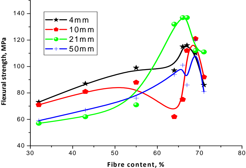
Fig. 6. Flexural strength of basalt short fibre composites.
