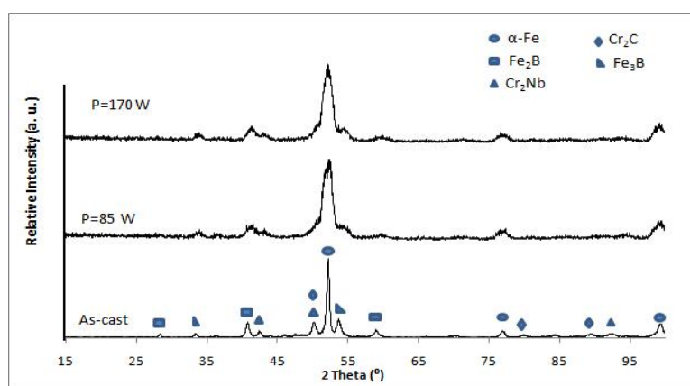
Fig. 4. XRD patterns of as-cast alloy, samples A1 and A3.
