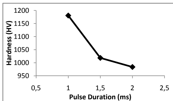
Fig. 5. Average hardness of all samples with different pulse durations.
