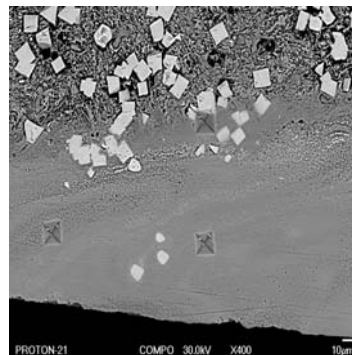
Fig. 3. FESEM micrograph of the processed zone.
