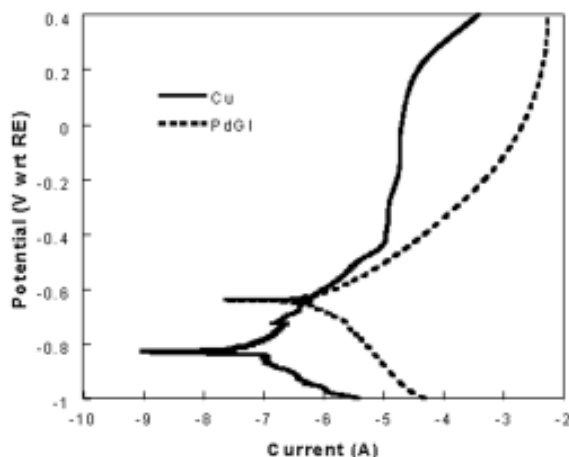
Fig. 2. Polarization curves for the anodic oxidation of ethylene glycol solution containing 2 mol/l NaOH on different substrates.
