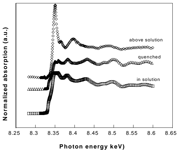
Fig. 7. X-ray Ni edge absorption spectra of FeNi films deposited on Cu substrate. When the substrate was suspended above solution, the sharp peak near the absorption edge (photon energy =8.35 keV) indicated Ni oxidation.
