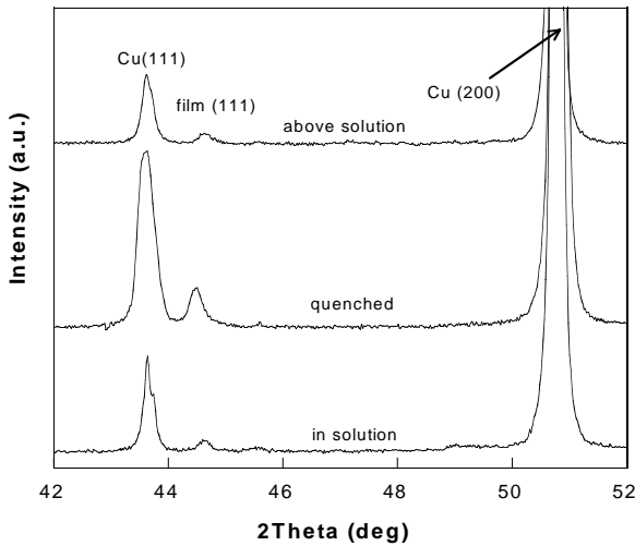
Fig. 5. XRD patterns of FeNi films deposited on Cu substrates. Only one film peak at 2\theta = 44.6^\circ was detected.
