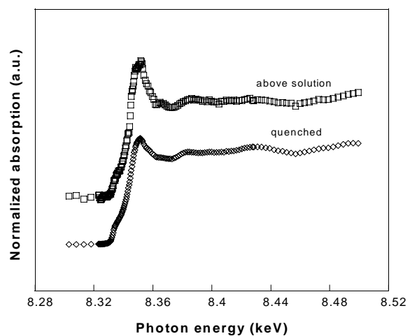
Fig. 8. X-ray Ni edge absorption spectra of FeNi films deposited on PdGI substrate. Both samples had been apparently oxidized.
