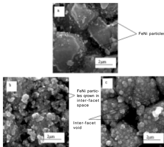
Fig. 4. SEM micrographs of FeNi film deposited on PdGI substrate (a) quenched with deposition time 20min; (b) quenched with deposition time 60min; (c) above solution with deposition time 60min.
