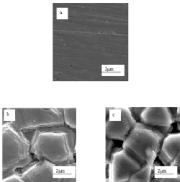
Fig. 1. SEM micrographs of Cu and etched glass substrates (a) Cu substrate; (b) 25 nm Pd film sputtered on etched glass; (c) 2 nm Au film sputtered on etched glass.
